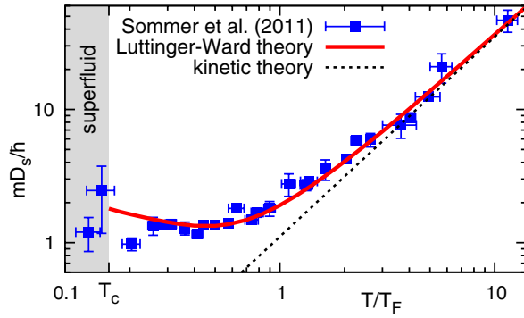
FIG. 1 (color online). Spin diffusivity D_s vs reduced temperature T/T_F (solid red line) in the normal phase, T > T_c \simeq 0.16T_F . The experimental data [4] (blue squares) for the trapped gas are rescaled down by a factor of 4.7 to compensate for the effect of the trapping potential. The dashed black line is the result from kinetic theory, D_s = 1.1(T/T_F)^{3/2}\hbar/m .
