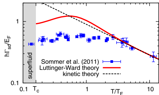
FIG. 3 (color online). Spin drag rate \Gamma_{sd} (in units of E_F/\hbar ) vs reduced temperature T/T_F (solid red line). The experimental data [4] (blue squares) for a trapped gas are rescaled up by a factor of 5.3 to compensate for the effect of the trapping potential. The dashed black line is the result from kinetic theory, \Gamma_{sd} = 0.9(T/T_F)^{-1/2}E_F/\hbar .
