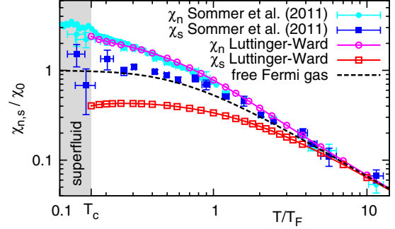
FIG. 4 (color online). Compressibility \chi_n (circles) and spin susceptibility \chi_s (squares) vs reduced temperature T/T_F . The experimental data [4] (full symbols) are compared to our Luttinger-Ward calculation (open symbols). The dashed black line is the susceptibility of the free Fermi gas.
