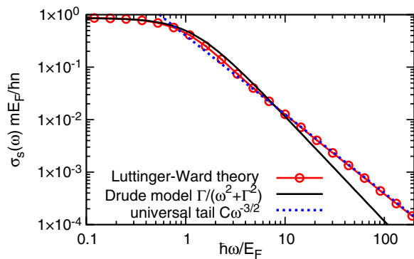
FIG. 2 (color online). Spin conductivity \sigma_s(\omega) (in units of \hbar n/mE_F ) vs frequency (red circles) at T = 0.5T_F . The Drude model (solid black line) has the same total spectral weight as \sigma_s(\omega) given by the spin f -sum rule. Part of the spectral weight is transferred from lower frequencies into a universal high-frequency tail (dotted blue line) \sigma_s(\omega \rightarrow \infty) = C/3\pi(m\omega)^{3/2} with Tan contact density C = 0.086k_F^4 [9].
