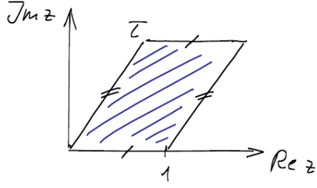
Figure 21: Torus defined as \mathbb{C}/\mathbb{Z}^2 .
