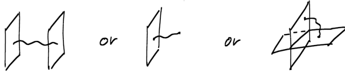
Figure 10: Various brane configurations with strings attached.
