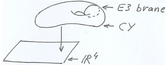
Figure 27: An E3-brane instanton, corresponding to a euclidean D3 brane wrapped on a 4-cycle of a CY over one of the points of the non-compact space-time \mathbb{R}^4 .
