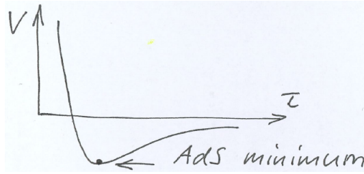
Figure 28: Qualitative behaviour of the scalar potential arising after the inclusion instanton or gaugino condensation effects.
