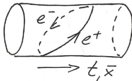
Figure 23: Effective instanton arising from a particle-antiparticle fluctuation warping the compact space of an S^1 compactification (figure from [76]).
