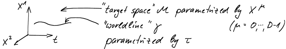
Figure 6: Point particle through target space.
