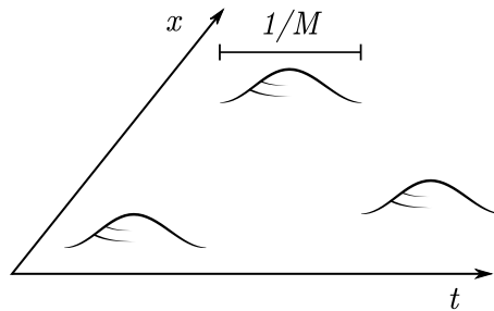
Figure 22: Instantons as localized lumps of field strength (figure from [76]).
