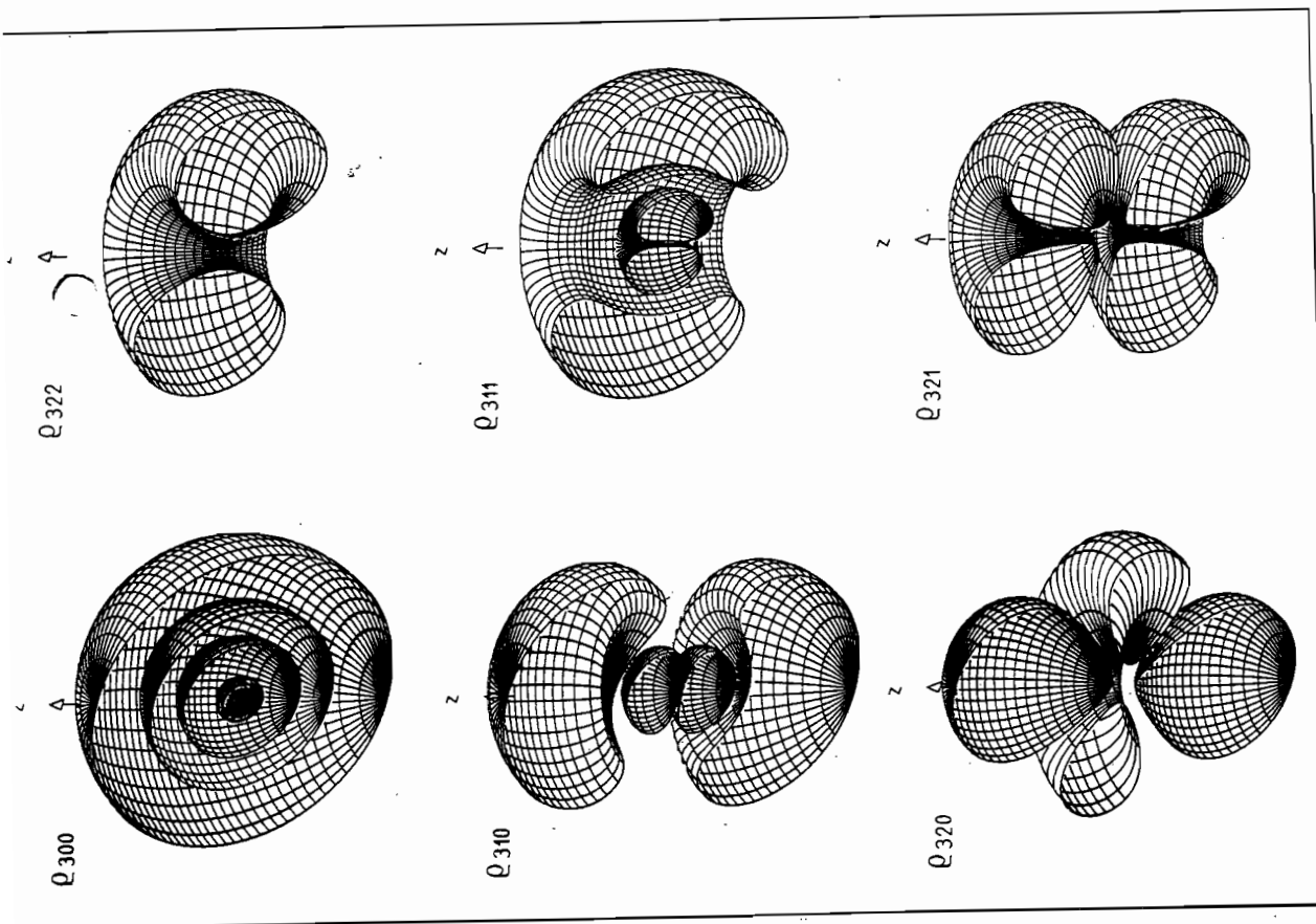
Fig. 13.21. Surfaces of constant probability density \rho_{3l_m} = 0.0002 in the half-space x > 0 .
