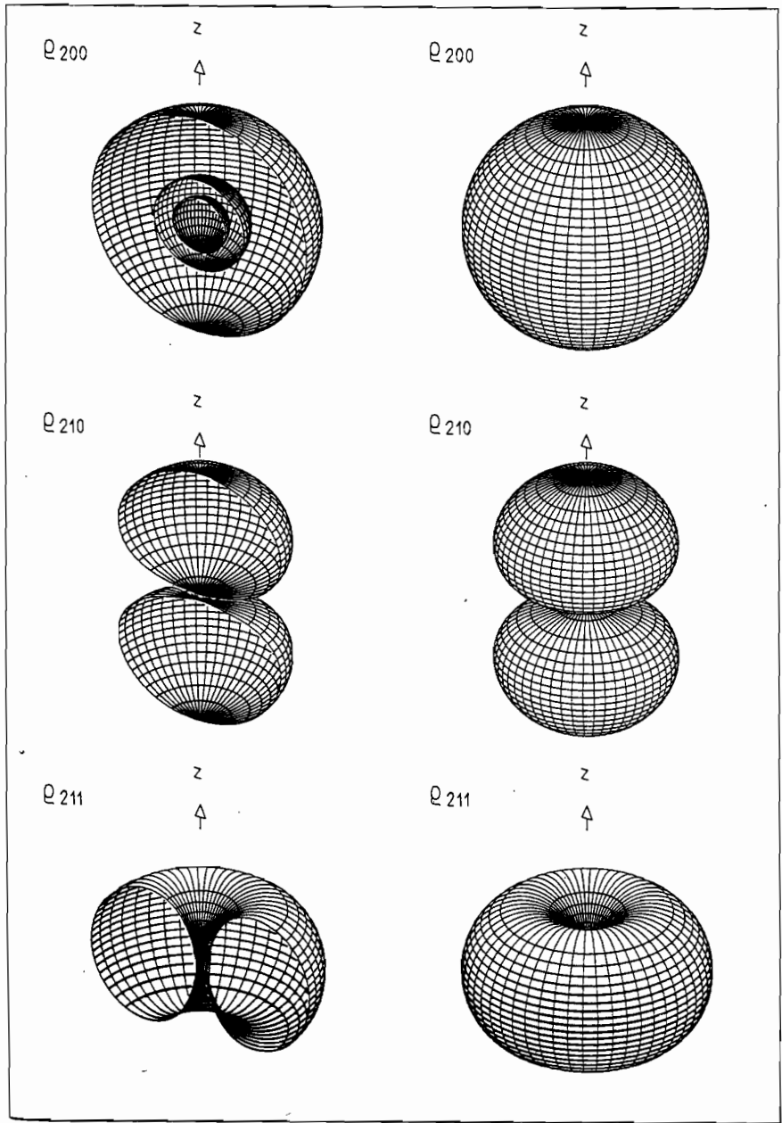
Fig. 13.18. Surfaces of constant probability density \rho_{2lm} = 0.02 in full x, y, z space (right) and in the half-space x > 0 (left).
